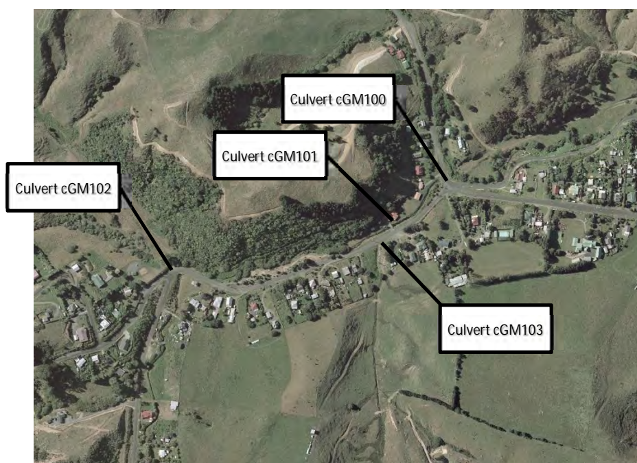
Figure 4: Culvert locations
